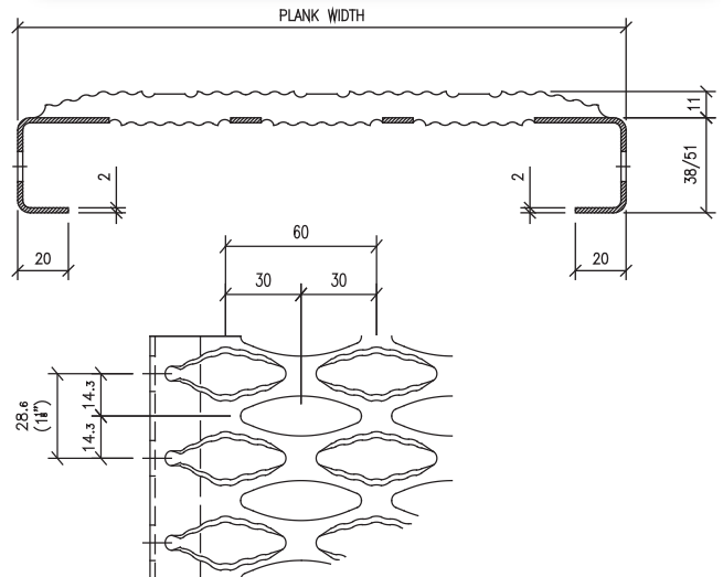
Aluminium/Stainless Steel
